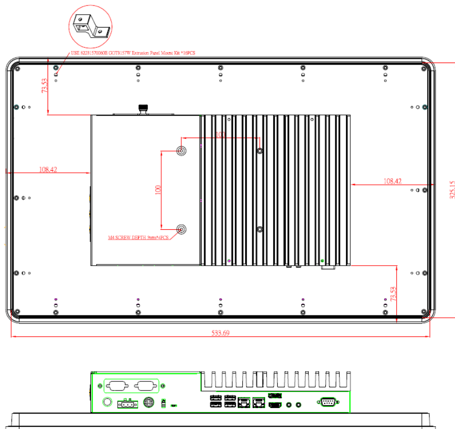
Diagram 1-2 Back outline of the GOT321W-502-PCT
