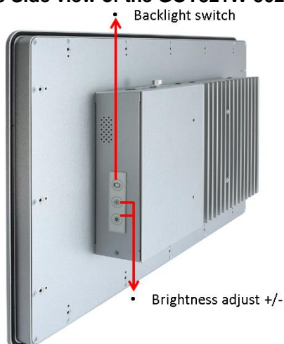
Figure 1-3 Side view of the GOT321W-502-PCT
