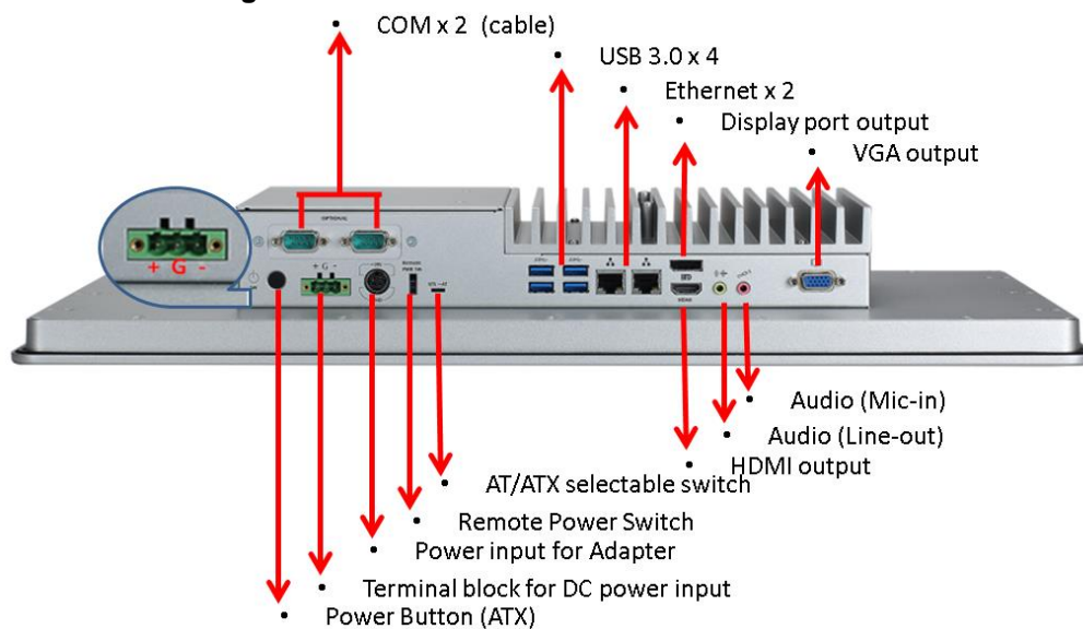
Figure 1-2 Bottom view of the GOT321W-502-PCT
