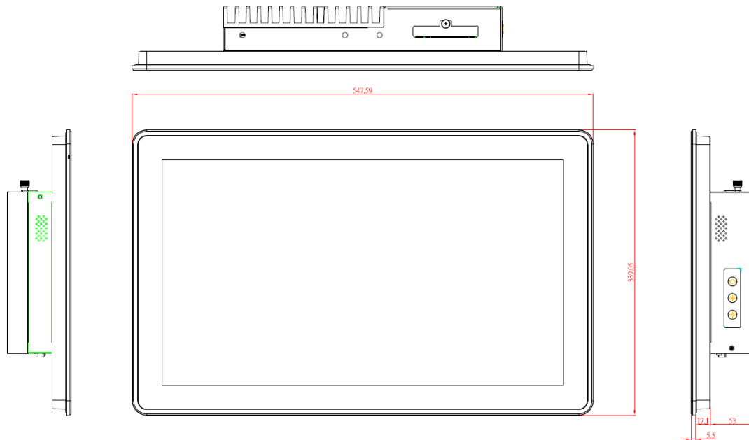
Diagram 1-1 Front dimensions and outline of the GOT321W-502-PCT
