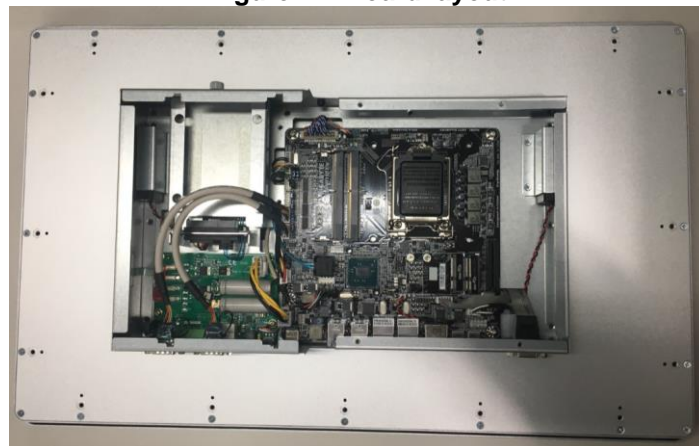
Figure 2-2 Board layout
